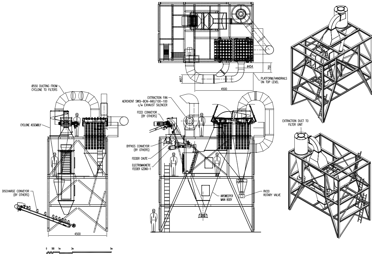
Typical air classifier arrangement
